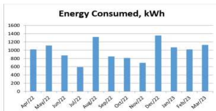
Chart No 2: Variation in Monthly Energy Consumption:
