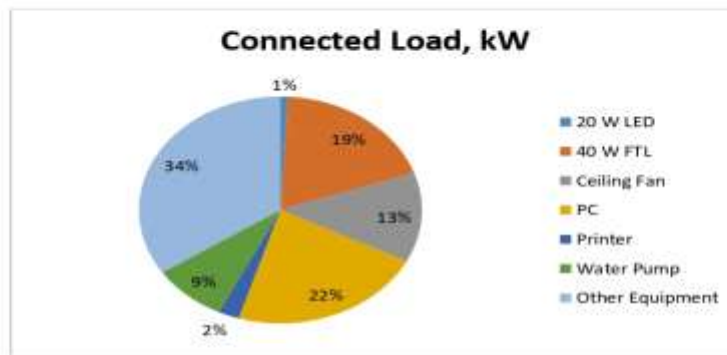
Chart No 1: Study of Connected Load:
